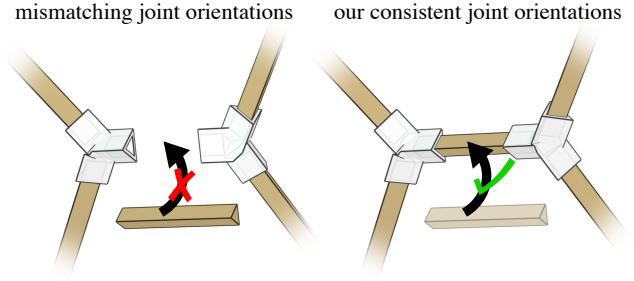
Figure 17: Direct extensions of wiremeshing algorithms (e.g., [PRW*19, Har06]) may result in twisting along edges, leading to inconsistent rod-orientations at either end. Our joint-construction algorithm avoids this.
