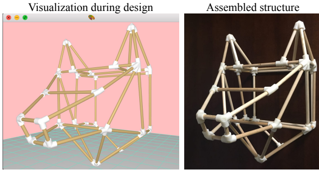
Figure 3: RSDesigner displays a visualization closely matching the eventual fabrication, reducing surprise at assembly time.
