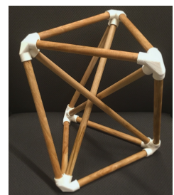
Figure 11: A close fit.
