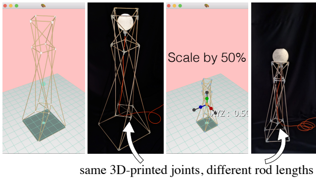
Figure 12: Isotropic scaling the design will not change the joint geometry, so the same 3D prints may be reused at different scales.
