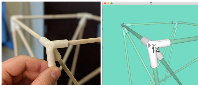
Figure 10: The joint geometries shown by RSAssembler match the 3D printed. Engraved joint IDs also facilitate orientation matching.
