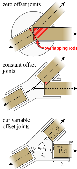
Figure 16: Previous joint geometry generation methods do not consider the possibility of rod intersections at joints. A per-edge offset is necessary and can be minimized on a case-by-case basis.
